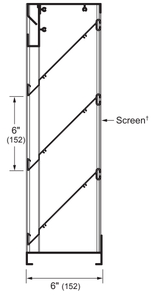
Vertical Section
